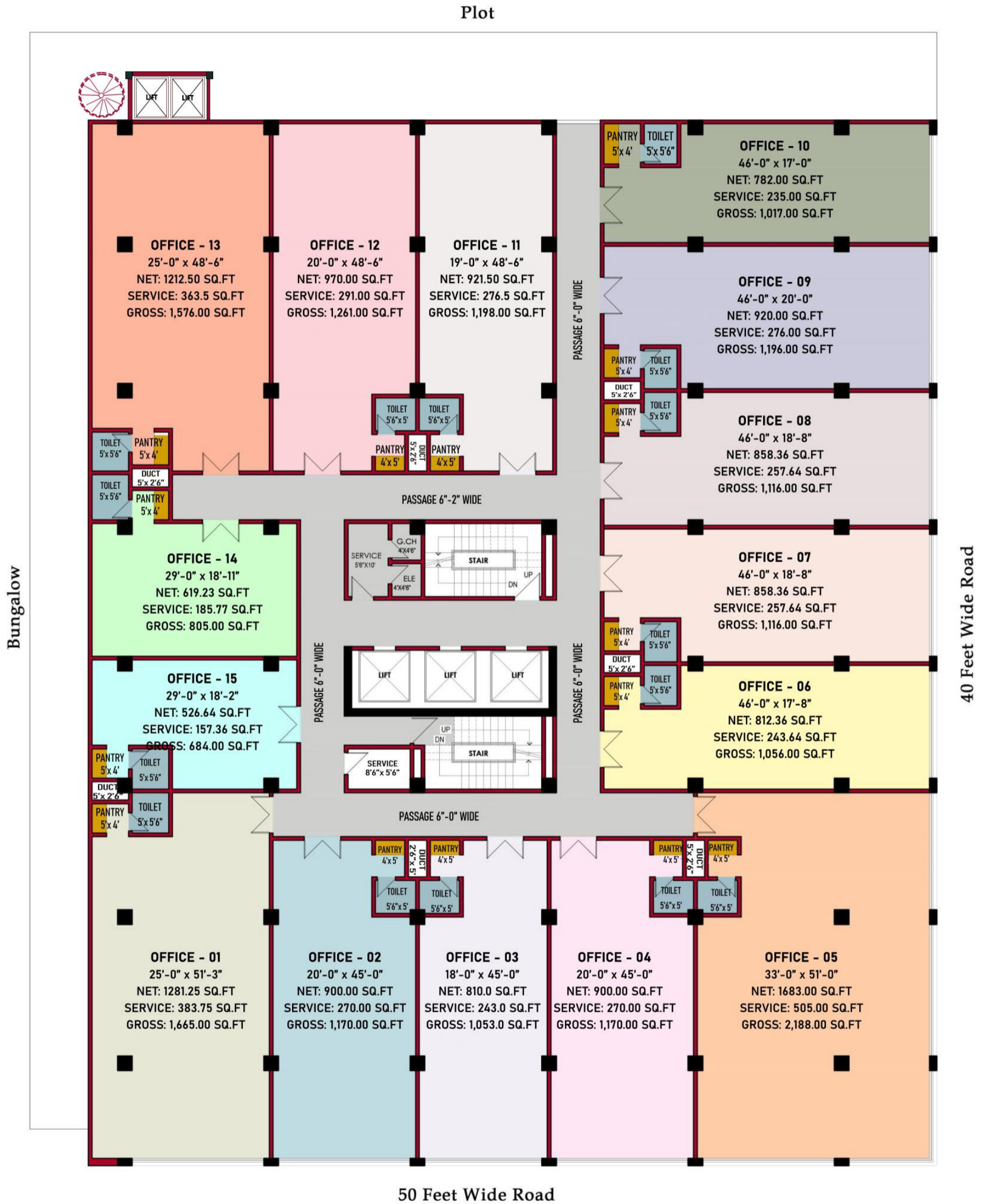
1st to 4th Floor Plan
